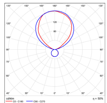
Polar curve for 3x1340 lumen LED strips with clear diffuser up and opal down.
